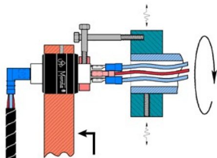
Fixed Support Vibration isolating mount with floating drive coupling.
