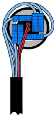
Terminal connector layout for Model 830 (stationary end).
